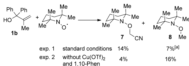
Scheme 5. Trapping experiments with 2,2,6,6-tetramethylpiperidin-1-oxyl (TEMPO). [a] Yield based on TEMPO.
