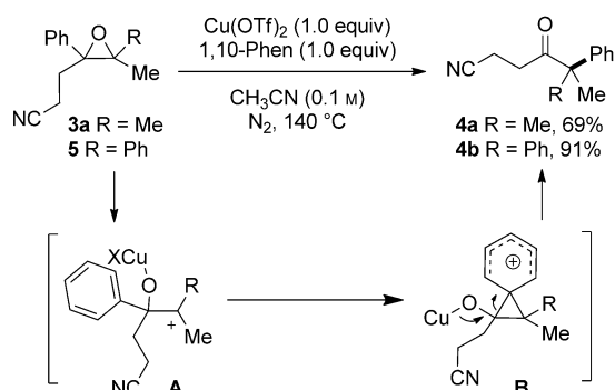
Scheme 3. Cu(OTf) 2 -promoted rearrangement of epoxides 3a and 5 .
