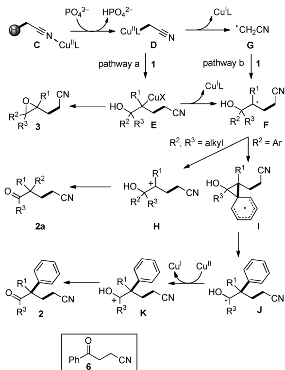
Scheme 4. Possible reaction pathways of the copper-catalyzed coupling reaction of allylic alcohols with alkyl nitriles to give ketones 2 .
